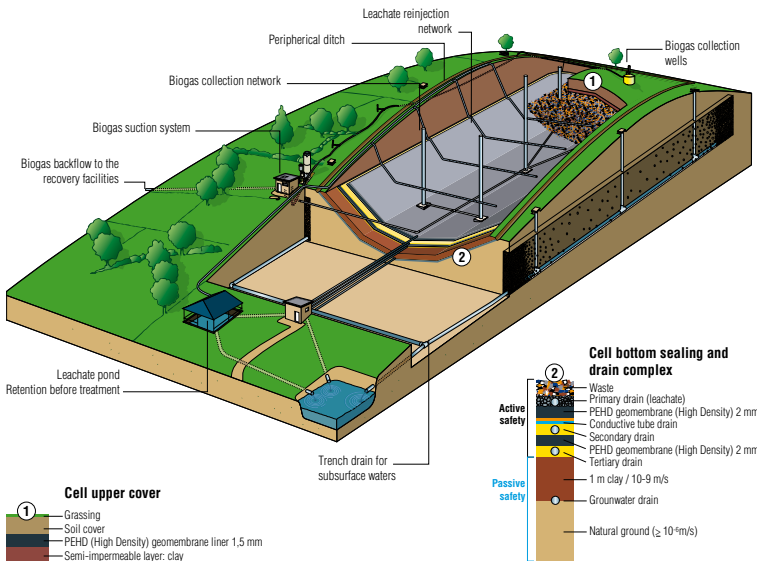
Graphic representation of non-hazardous waste landfill
